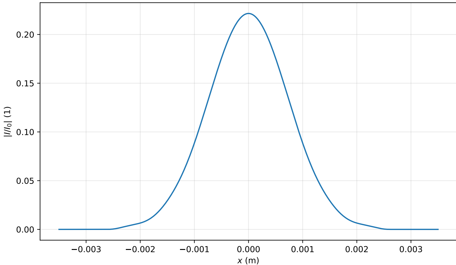
Intensity profile I(x, y = 0, z = 3.981m)/I_0 , P_{in}=0.1P_{cr} , artificial time
